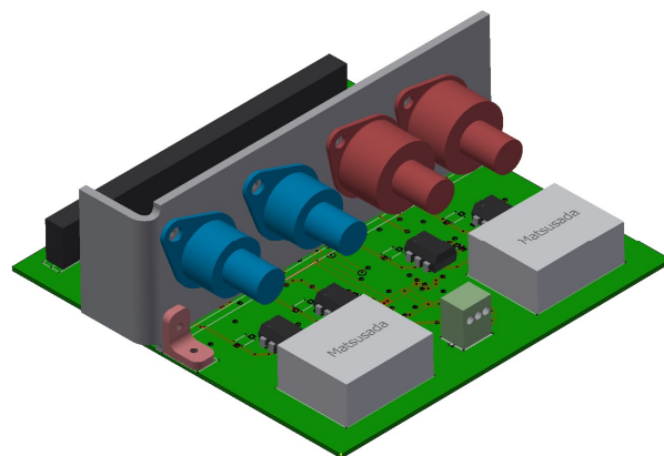
FIG. 1. 3D model of detector assembly (DA). The PCB has the form factor of a cubesat and contains four APDs: two SLiKs and two C30902SHs from Excelitas, two high-voltage (HV) modules, two discriminators, one thermoelectric cooler (TEC) controller, two pulse processing circuitries, and several electrical switches to select HV supplies and TECs. The electrical platform is controllable by processor, which is interfaced through PC/104— an embedded computer standard connector. [Figure is by Shubham Singh 3 ]
