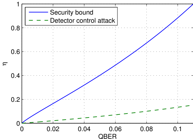
FIG. 5. (Color online) Comparison of the detector control attack and the bound from the security proof [16]. The region to the left of the security bound curve (solid curve) allows extraction a secure key. The region to the right of the detector control attack curve (dashed curve) is clearly insecure, because the attack presented in Sec. II can be applied. The region between the curves should be assumed insecure.
