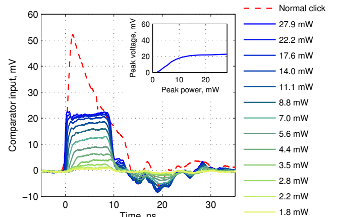
FIG. 3. (Color online) Electrical response in the latched state to the 10\ \text{ns} , 1550\ \text{nm} optical trigger pulse. All traces are averaged over 500 samples. The trigger pulse saturates at an electrical response of about 20\ \text{mV} (see inset), compared to the normal detection event which reaches peak amplitude of about 50\ \text{mV} .
