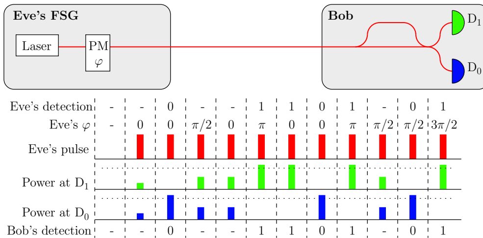
Figure 2. Detector control in a DPS implementation: Eve's FSG consists of a laser source producing a train of coherent pulses with amplitude P_{\text{always}} , and a phase modulator (PM). Eve controllably causes identical detection events in Bob by an appropriate phase \varphi in each pulse. No trigger pulse is applied to the left of the diagram, nor in the first slot. (The color version of this figure is included in the online version of the journal.)
