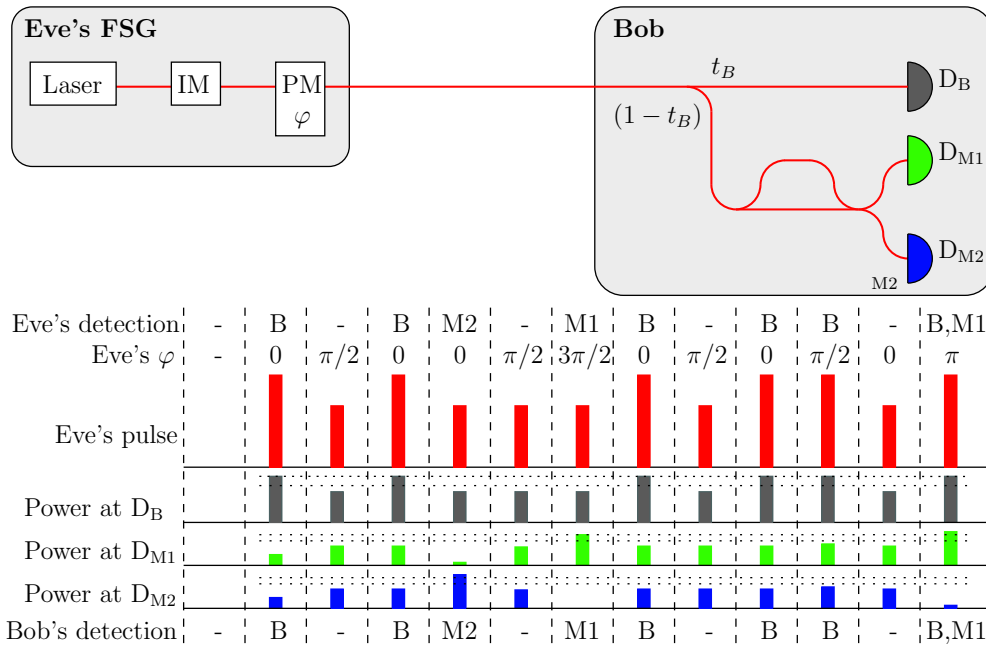
Figure 3. Detector control in a COW implementation: Eve's FSG consists of a laser source producing a train of coherent pulses, an intensity modulator (IM) and a phase modulator (PM). The lower part of the figure shows an example of detector control, where the system parameters are assumed to be t_B=0.5 , P_{\text{never},M}=400\ \mu\text{W} , P_{\text{always},M}=500\ \mu\text{W} , P_{\text{never},B}=600\ \mu\text{W} and P_{\text{always},B}=750\ \mu\text{W} . The dashed lines in the diagram are the detector thresholds. Eve controllably causes identical detection events in Bob by an appropriate phase \varphi and amplitude in each pulse. The trigger pulse amplitude is 2P_{\text{always},M}=1000\ \mu\text{W} , and is increased to 2P_{\text{always},B}=1500\ \mu\text{W} to trigger the data detector. No trigger pulse is applied to the left of the diagram, nor in the first slot. (The color version of this figure is included in the online version of the journal.)
