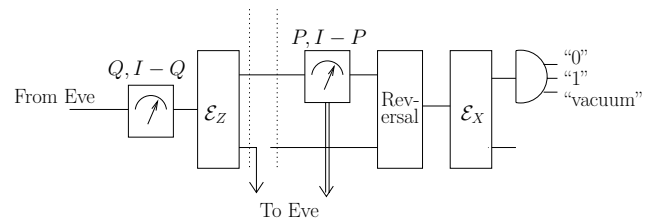
FIG. 2. Bob's setup for virtual X -basis prediction. The optical and electronic modes are denoted by a single line in this figure.
