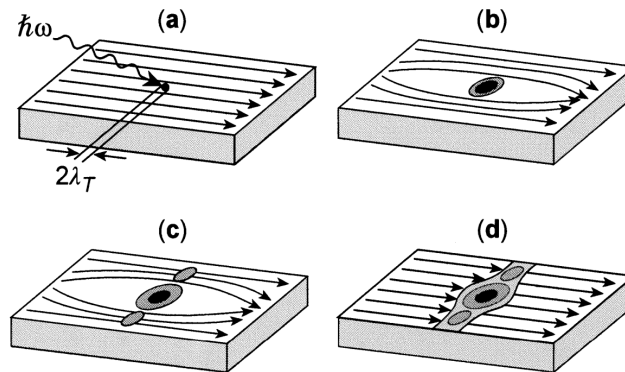
Figure 4.3: Single photon detection using a superconducting nanowire. (a) A photon is absorbed in the superconducting nanowire, and causes a normally conducting hot-spot. (b) The bias current circumvents the hot-spot, increasing the current density outside the hot-spot. (c) The current density on each side of the hot-spot exceeds the critical current density, and a larger piece of the cross-section is now normally conductive. (d) The normally resistive region covers a whole cross-section of the nanowire, which now has a non-zero resistance. Reprinted from Reference [113], ©2003 IEEE.
