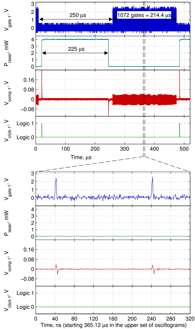
Fig. 7. Thermal blinding of frames. The oscillograms show electrical and optical signals when frames of 1072 gates in detector 1 are thermally blinded by a 225 μs blinding pulse, with 3.5 mW pulse power at detector 0, and 4 mW pulse power at detector 1. The blinding pulse causes a detection event outside the frame, where the system probably does not register clicks (If the click is registered, it could easily be avoided by increasing the power of the blinding pulse gradually, such that the comparator input AC-coupling keeps the voltage below the comparator threshold).
