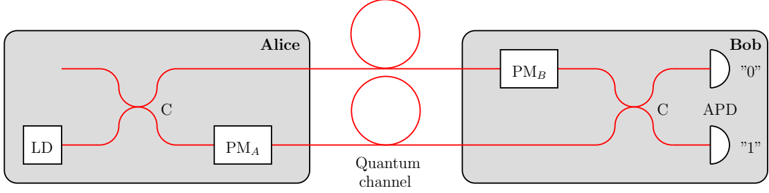
Figure 4.5: A phase encoded implementation using active basis choice. Alice randomly chooses a phase shift \varphi_A \in \{0, \pi/2, \pi, 3\pi/2\} to encode one of the four states. Bob randomly chooses a phase shift \varphi_B \in \{0, \pi/2\} to select his measurement basis. This setup is topologically equal to the polarization encoded system in Figure 4.4. LD: laser diode; C: fiber-optic coupler; PM_A : Alice's phase modulator; PM_B : Bob's phase modulator; APD: avalanche photodiode.
