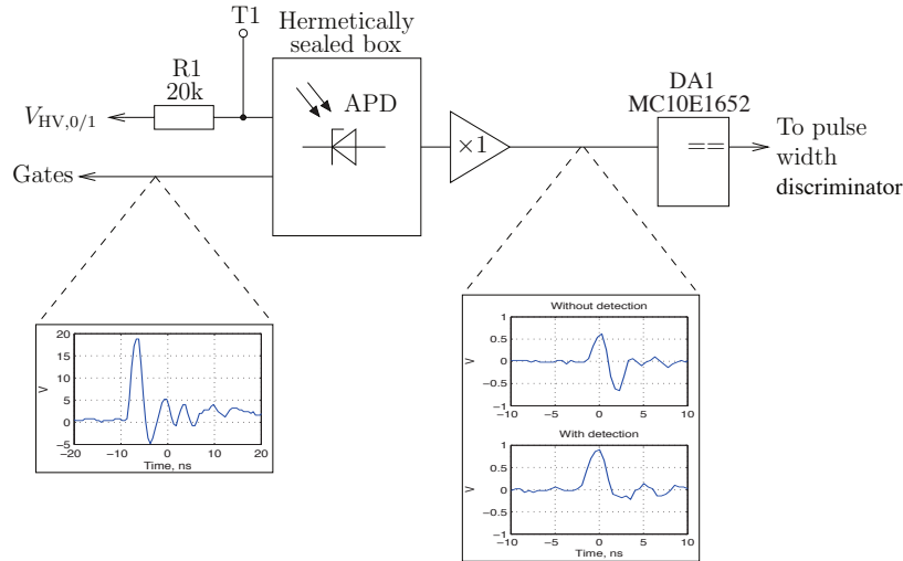
FIG. 2. Schematics of the detection circuit in QPN 5505 based on reverse engineering. Tap T1: analog tap of the APD bias voltage ( V_{bias,0/1} ). The APD as well as parts of the circuit are inside a hermetically sealed box (HSB). The bias voltage from a high voltage supply is connected to the HSB through the resistor R1 = R_{bias} = 20\text{ k}\Omega . For the settings which we used, V_{HV,0} = 41.86\text{ V} and V_{HV,1} = 41.41\text{ V} as measured in the circuit. The gates were applied to the HSB with an amplitude about 10 times larger than the setting in the control software. We do not know how the gates are mixed with the bias because this is done inside the HSB, which we decided not to open. The output of the HSB goes to an analog repeater and then a comparator DA1 which converts the APD output into pulses of different length corresponding to click/no click event. In the experiment, we simply used the QKD software to measure the detector count.
