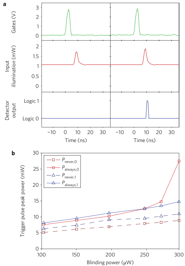
Figure 4 | Detector control. a , Electrical and optical signal oscillograms when detector 0 in Clavis2 is blinded by 1.08 mW c.w. illumination, and controlled by a superimposed 2.5-ns-long laser pulse timed slightly behind the gate (see Supplementary Section III for detailed measurement setup). The superimposed P_{never,0} = 647 \mu\text{W} (detector 1: P_{never,1} = 697 \mu\text{W} ) trigger pulse never causes a detection event, whereas the P_{always,0} = 808 \mu\text{W} ( P_{always,1} = 932 \mu\text{W} ) trigger pulse always causes a detection event. b , Click thresholds versus the applied c.w. blinding illumination for the QPN 5505. When the blinding power increases, P_{always,0} diverges, perhaps because the bias voltage is approaching the punch-through voltage of the APD (see Supplementary Section II).
