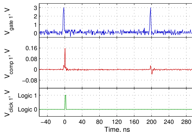
Fig. 3. An example of electrical signals during two gates in detector 1 without any illumination. In the first gate thermal fluctuations or trapped carriers have caused an avalanche, and a click at the comparator output (dark count). A typical amplitude of the avalanche peak is 200 mV for detector 0 and 300 mV for detector 1. Normally the system removes 50 gates after a detection event, but for this oscillogram this feature has been disabled. In the second gate there is no detection event. When no current runs through the APD, it is equivalent to a capacitor, and thus approximately the derivative of the gate pulse shape propagates to the comparator input, with peak positive amplitude \approx 35 mV.
