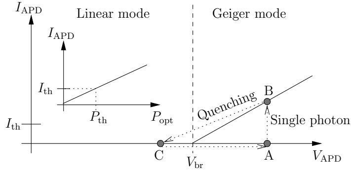
Figure 4.1: The operating principles of an APD. First the APD is biased at a point (A) above the breakdown voltage V_{br} . When a single photon arrives, it causes an electron-hole pair which amplifies to a macroscopic current (B). A photon arrival is signaled when the current exceeds the comparator threshold I_{th} . Afterwards, the current is stopped through quenching (C), before the voltage is brought back above the breakdown voltage again. For a bias below the breakdown voltage, the current through the APD depends linearly on the optical power incident on the APD.
