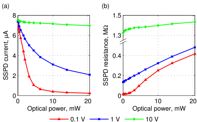
FIG. 2. (Color online) Response to continuous-wave (CW) light in the latched state. (a) Current I through the SSPD vs. optical power at 1550\ \text{nm} , at different voltages V applied across the SSPD. (b) SSPD resistance R = V/I .
