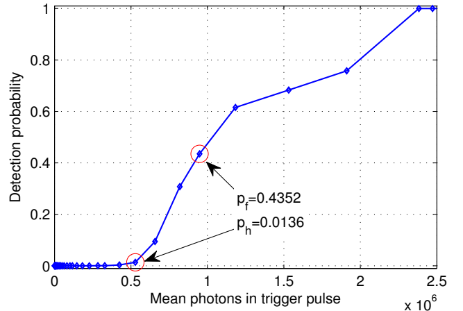
FIG. 1. (Color online) The detection probability versus mean photon number in the trigger pulse for the SSPD in Ref. [36], at 1550 nm and I_b = 0.8I_c . Count rates were extracted from Fig. 1 in Ref. [36], and divided by the pulse repetition frequency of 82 MHz to obtain the detection probability. The red circled data points were used to calculate the QBER and the transmittance from an attack.
