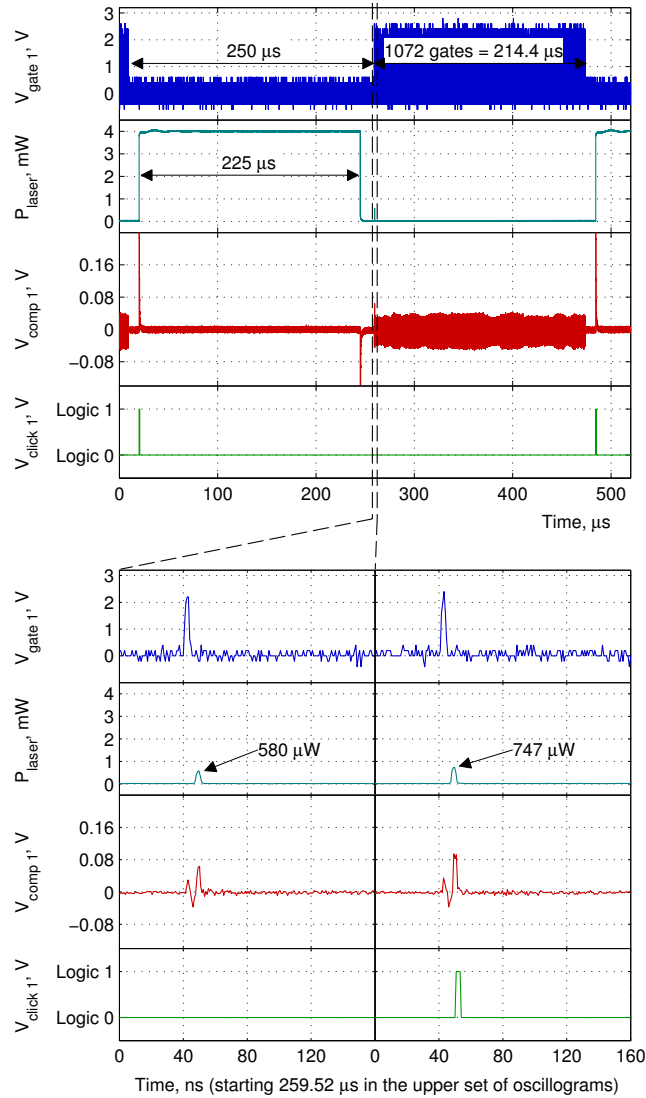
Fig. 8. Detector control during thermal blinding of frames. The oscillograms show electrical and optical signals when frames of 1072 gates in detector 1 are thermally blinded by a 225 μs blinding pulse, with 3.5 mW pulse power at detector 0, and 4 mW pulse power at detector 1, and the detector is controlled by a 4 ns long control pulse timed slightly after the second gate in the frame. In the upper and lower left sets of oscillograms, the 580 μW control pulse never causes any click. In the lower right set, the control pulse is applied after the same gate in the frame, but now its increased 747 μW peak power always causes a click.
