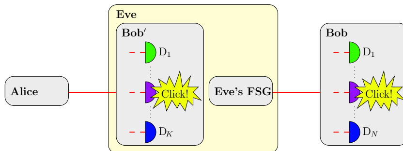
Figure 1. Scheme of a detector control attack: Eve measures the states from Alice using a copy of Bob’s measurement device (Bob’) to obtain a detection event. She then uses a faked-state generator (FSG) [42] to generate a bright pulse tailored to cause the same detection event in Bob. (The color version of this figure is included in the online version of the journal.)
