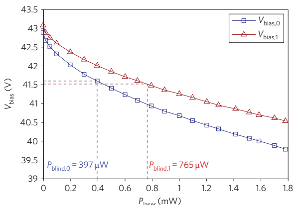
Figure 3 | Bias voltage at T1 versus c.w. laser power for Clavis2. Detector 0 is blind (dark count rate exactly zero) at P_{laser} > 397 \mu\text{W} , and detector 1 is blind at P_{laser} > 765 \mu\text{W} . QPN 5505 has similar characteristics; due to the larger value of R_{bias} , its detector 0 goes blind at P_{laser} > 60 \mu\text{W} and detector 1 goes blind at P_{laser} > 85 \mu\text{W} (see Supplementary Section II for more details of QPN 5505 blinding).
