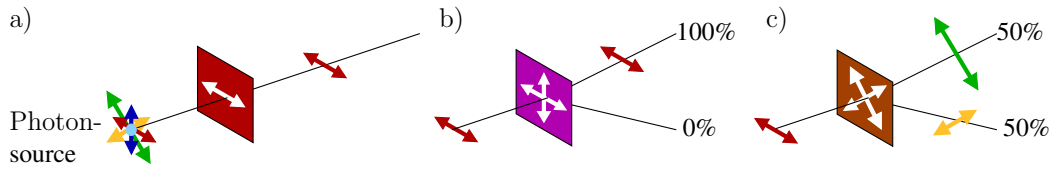
Figure 2.1: The components used for a simple polarization encoded BB84 scheme. a) A photon source is followed by a linear polarizer to generate a qubit with the desired polarization, in this case a horizontally polarized photon. b) When a horizontally polarized photon propagates through a horizontally oriented polarizing beam splitter (PBS), it is deterministically found in the exit of the beam splitter corresponding to the horizontal polarization. c) When a horizontally polarized photon propagates through a +45^\circ oriented PBS, the photon has 50% probability to be found in each exit (but the photon will only be detected in one of them!). Furthermore, if the photon is found in the \pm 45^\circ exit of the PBS, the photon will have a \pm 45^\circ polarization afterwards. Therefore, the measurement has changed the state of the photon.
