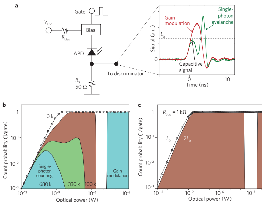
Figure 1 | InGaAs APD under CW illumination. The APD is thermo-electrically cooled to -30 °C and driven by voltage pulses of 3.5 ns, 4 V and 2 MHz. The excess bias is set to 2.5 V by the d.c. bias ( V_{\text{HV}} ) in the single-photon counting regime. A CW laser of wavelength 1.55 \mu\text{m} is used for illumination. a , A schematic for gated-mode operation and two APD output waveforms that trigger a photon click. b, c , Count probability against incident optical power for a biasing resistor ( R_{\text{bias}} ) of varying impedance ( b ) and for two differing discrimination levels, L_0 and 2L_0 ( c ).
